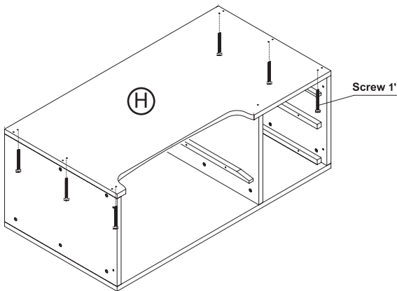
Bench Body
